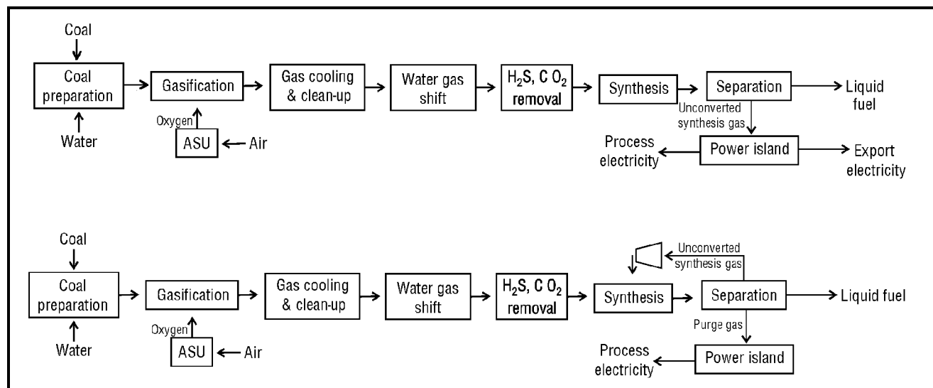
Figure B1. General system layout of making synthetic fuels from coal via gasification
